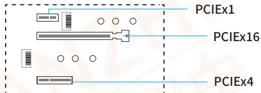
2-4 PCI Expansion Slot
