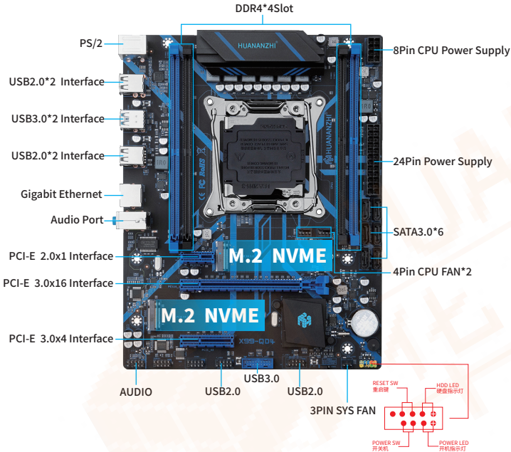
1-1 X99-QD4 Motherboard Illustration
